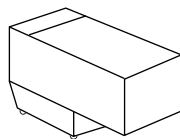
W 22" D 42" H 19" V633 CONSOLLE TABLE
